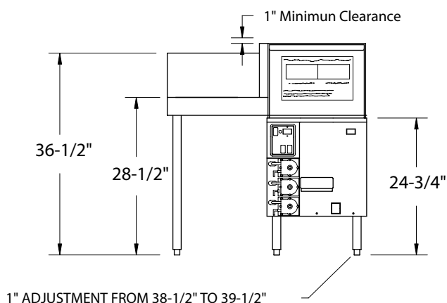
FRONT ELEVATION VIEWS
