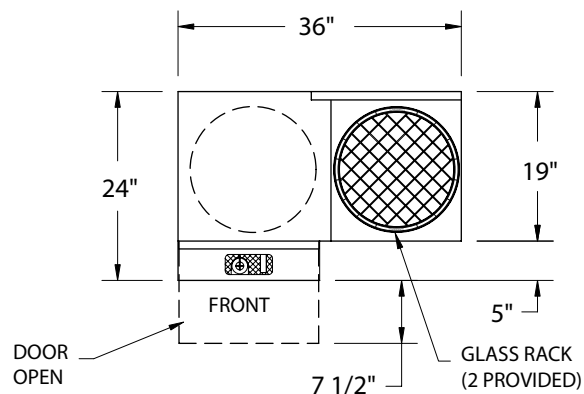
PLAN VIEWS
